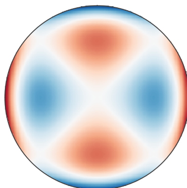
Secondary astigmatism
