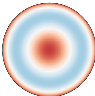
Primary spherical
