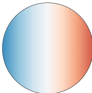
Cosine astigmatism
