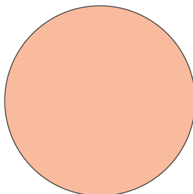
Defocus
