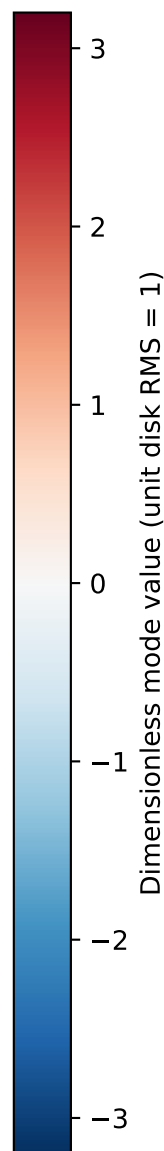
Secondary spherical
