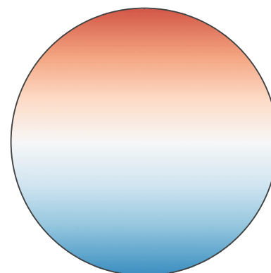
Sine astigmatism
